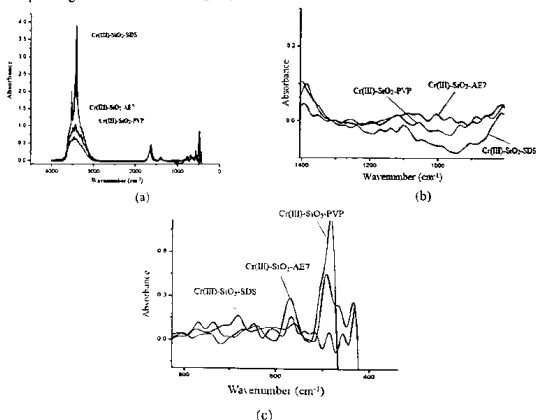
Figure 2 IR spectrum of passive Cr(III)- \text{SiO}_2 solution with different dispersing agents produced wavenumber range of 4000 - 400 \text{ cm}^{-1} (a); 1400 - 800 \text{ cm}^{-1} (b) and 800 - 400 \text{ cm}^{-1} (c)
