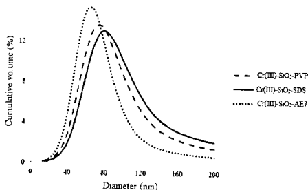
Figure 1 Particle-size distribution of nanosilica in passive solution containing dispersing auxiliaries.
