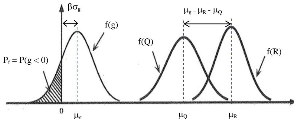
Figure 1. PDFs of load, resistance, and safety margin
