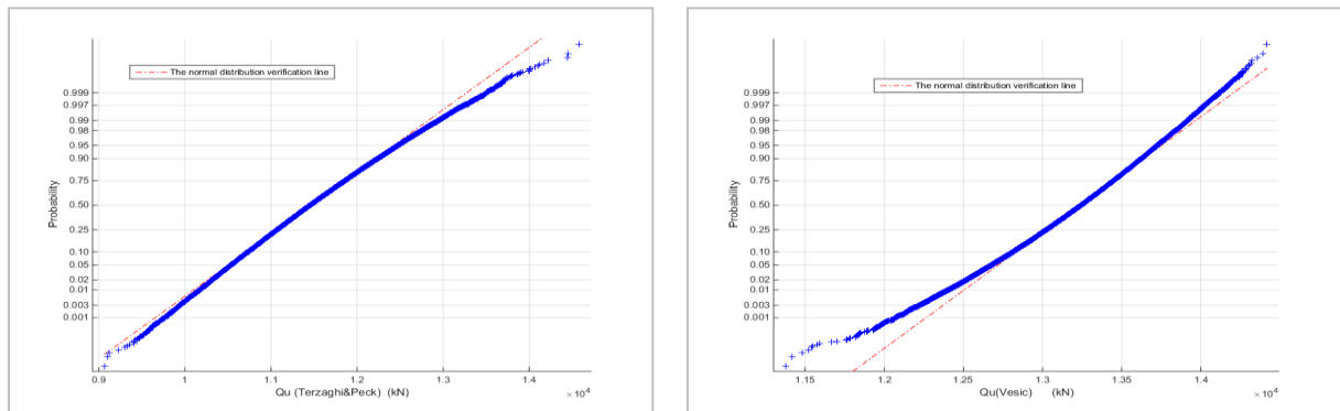
Figure 7. Normal distribution verification of the ultimate bearing capacity Q_{u(Terzaghi\&Peck)} and Q_{u(Vesic)} .
