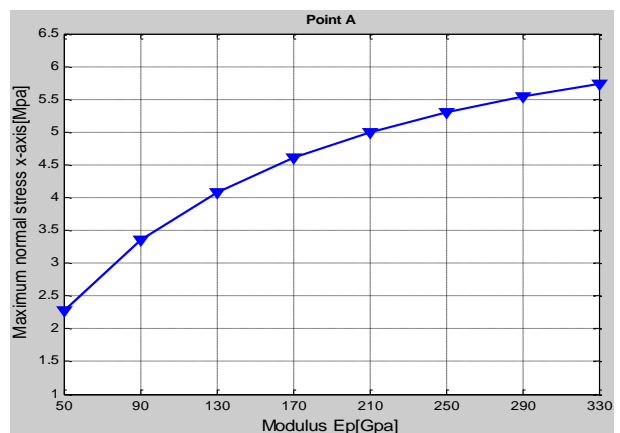
Figure 13. Correlation of \sigma_x^{\max} - E_p
