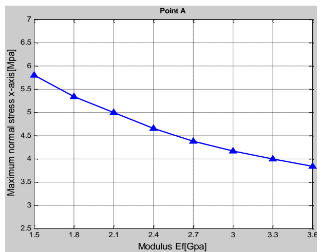
Figure 11. Correlation of \sigma_x^{\max} - E_f
