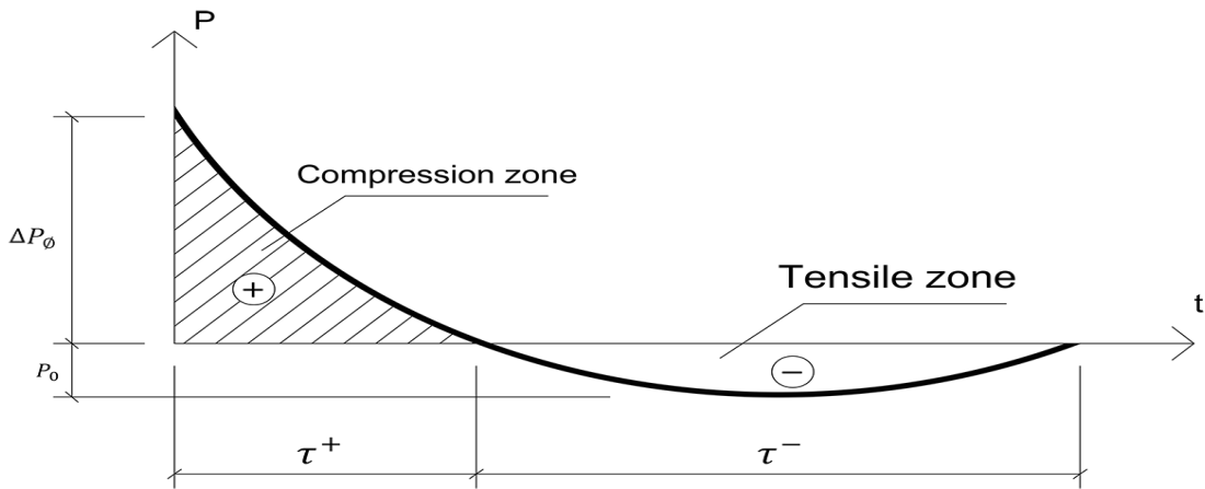
Figure 3. Shockwaves diagram
