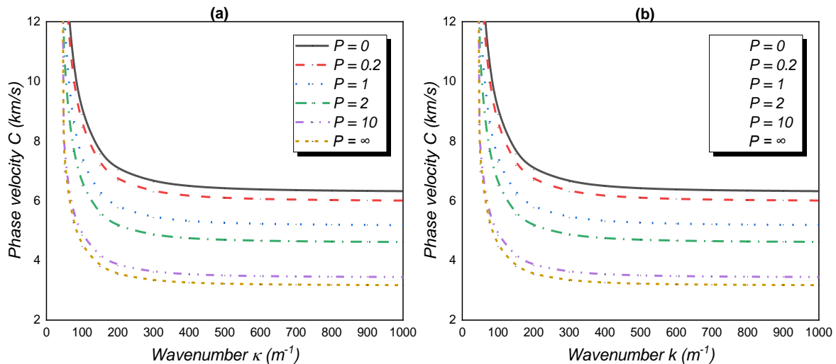
Figure 3. The dispersion relation between C and \kappa of FG porous shells: (a) spherical shell, (b) cylindrical shell
