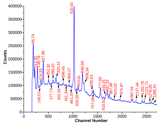
Fig. 5. Prompt gamma spectrum of ^{239}\text{U}
