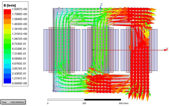
Figure 7. Vector distribution of the flux density at t = 500\text{ms}
