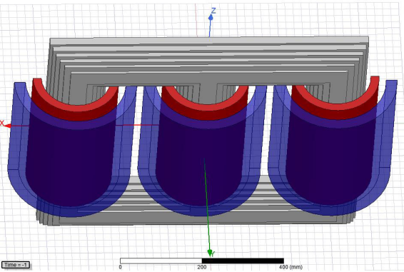
Figure 4. Transformer model used in Ansyes Maxwell 3D
