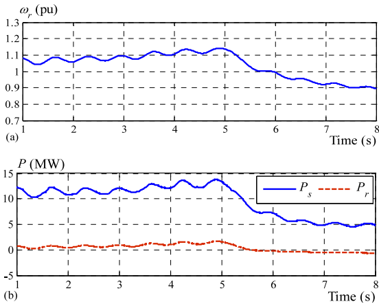
Figure 11. Chart of speed (a) and active power (b) of BDFIG-RT.
