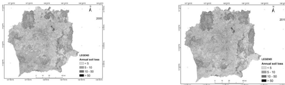
Figure 6. Actual soil erosion in Pleiku in 2005 (ton/ha/year)
