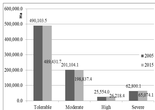
Figure 16. Changes in areas of SES in the Pleiku during 2005 - 2015
