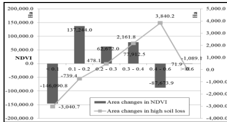
Figure 9. Relationship between area changes in NDVI and those in high soil erosion
