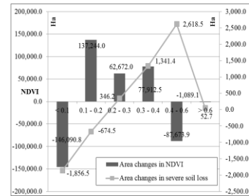
Figure 15. Relationship between area changes in NDVI and those in severe SES
