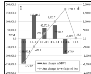
Figure 10. Relationship between area changes in NDVI and in very high soil erosion
