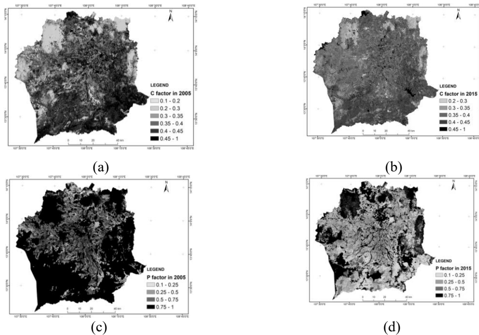
Figure 5. The cover management factor in 2005 (a), 2015 (b) and the conversion practice factor in 2005 (c), 2015 (d)
