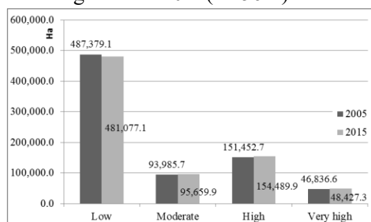
Figure 8. Changes in areas of the actual soil erosion classes in Pleiku during 2005 - 2015
