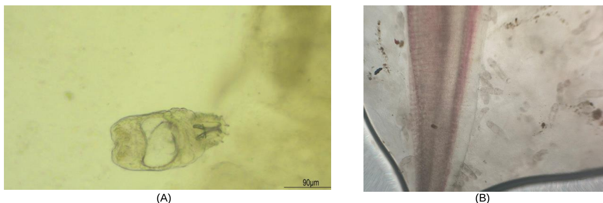
Figure 1. Gyrodactylus sp. parasitizing the (A) skin and (B) gills of rainbow trout ( O. mykiss ) cultured in a low-head RAS.
