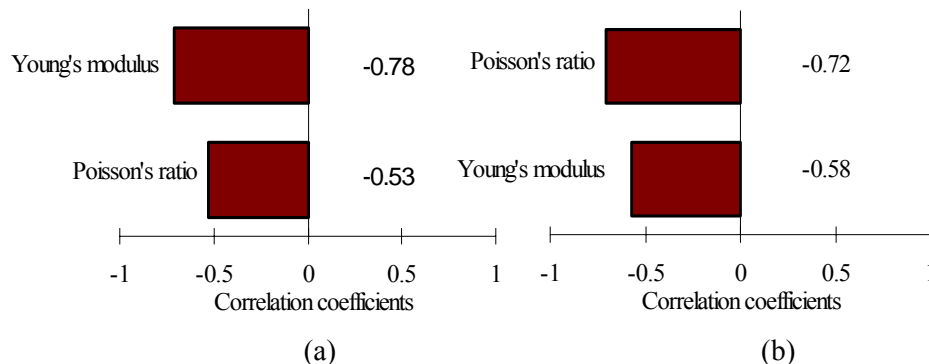
Figure 8. Tornado plot for (a) compaction, (b) subsidence.
