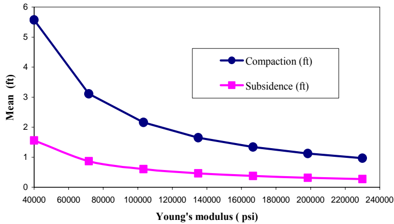
Figure 5. The impact of Young’s modulus on compaction and subsidence
