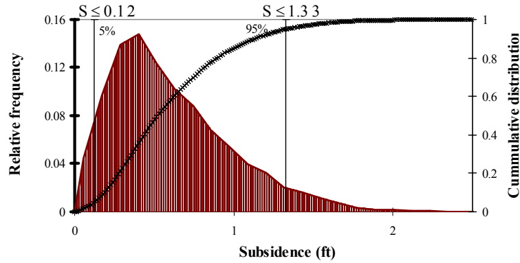
Figure 7: Subsidence uncertainty for experiment-3. The mean of Young’s modulus used in the experiment-3 is 86,508.81psi and a standard deviation is 41,17psi. Poisson’s ratio distribution has a mean of 0.29 and a standard deviation of 0.09
