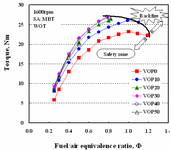
Fig. 5 Brake torque as a function of fuel-air equivalence ratio for each VOP
