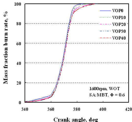
Fig. 7 Mass fraction burned rate versus crank angle
