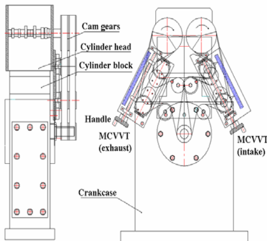
Fig. 1 Structure of the hydrogen-fueled engine
