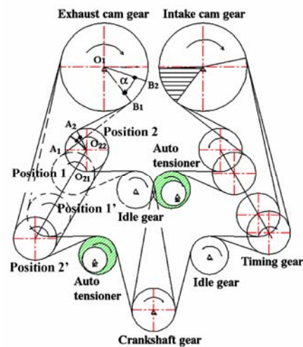
Fig. 2 Schematic diagram of MCVVT system
