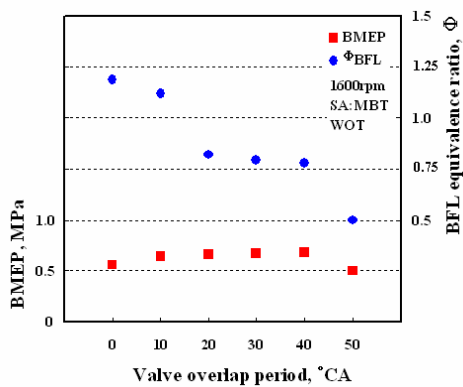
Fig. 9 Variation of BFL equivalence ratio and BMEP with respect to VOP
