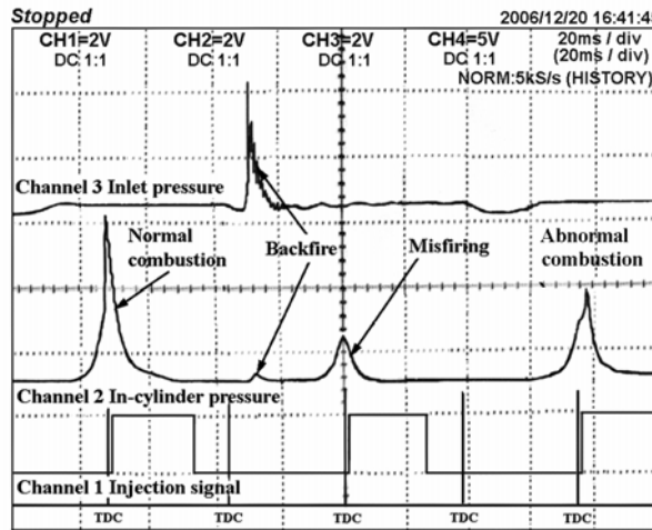
Fig. 8 Examples of backfire occurrence
