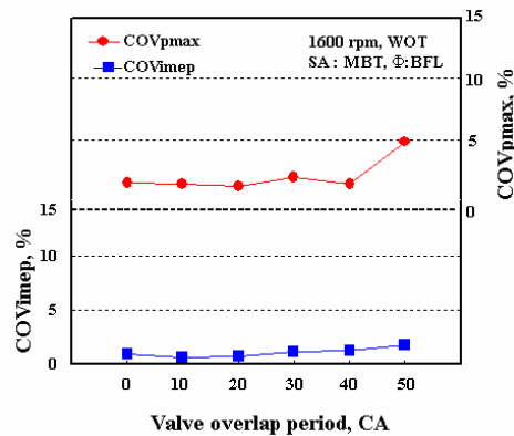
Fig. 10 COVimep and COVpmax versus VOP at \phi - BFL equivalence ratio
