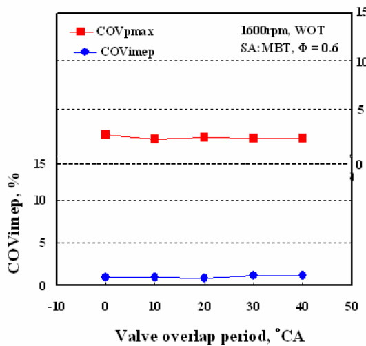
Fig. 4 COVimep and COVpmax versus VOP
