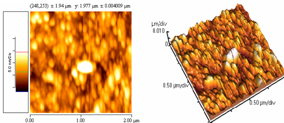
Hình 1b. \text{TiO}_2\text{-SiO}_2 (22.22 % \text{SiO}_2 ) : Rms Rough: 3.017 nm;
