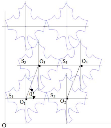
Fig. 4. Position of 4 pieces in the layout scheme
