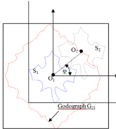
Fig. 5. Godograph of the piece
