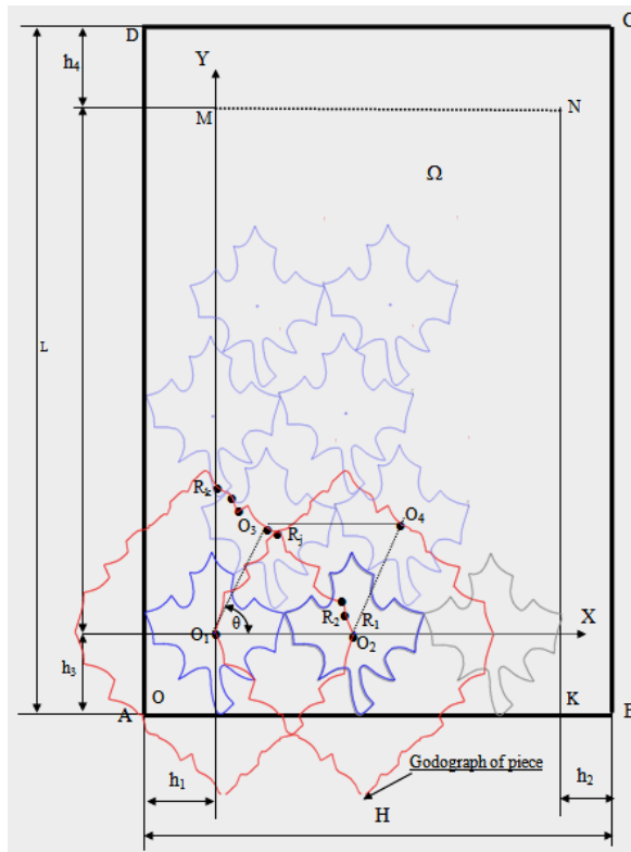
Fig. 6. Arrangement of oriented pieces on sheet material
