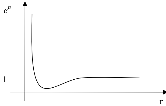
Fig.1. the graphic of function e^n
