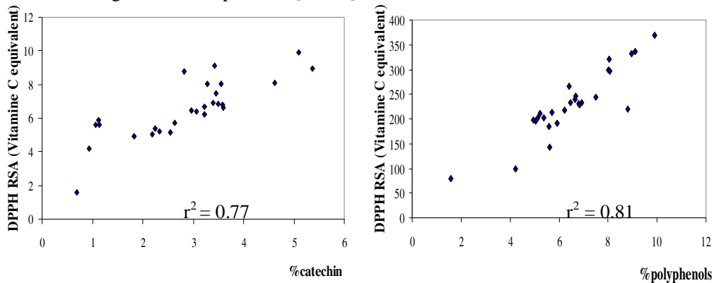
Figure 3.3. Relationship of catechins and polyphenols content to DPPH RSA
