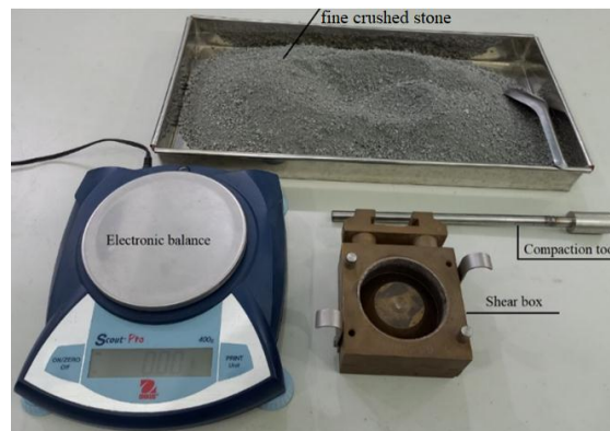
Figure 2. Fine crushed stone at the quarry in Phu Ly - Ha Nam and experiment tools.
