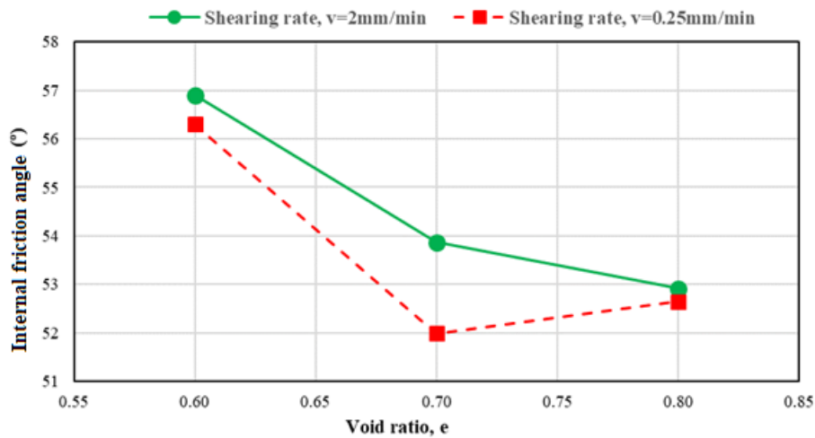
Figure 8. Effect of void ratio on internal friction angle of fine crushed stone.
