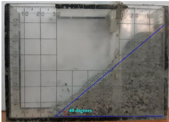
Figure 4. Determining the angle of repose of the fine crushed stone.
