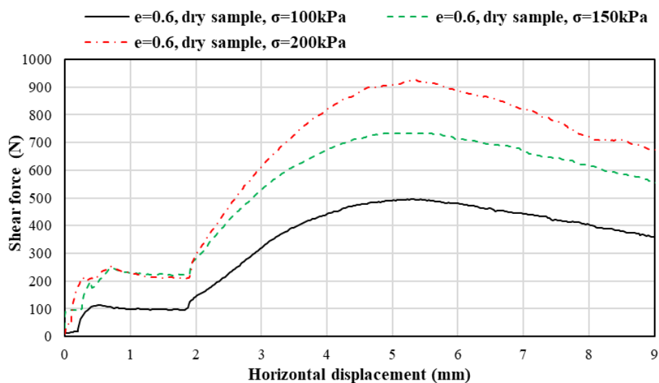
Figure 6. Relationship of shear force and horizontal displacement (dry sample, void ratio e = 0.6 , shearing rate 0.25 mm/min).
