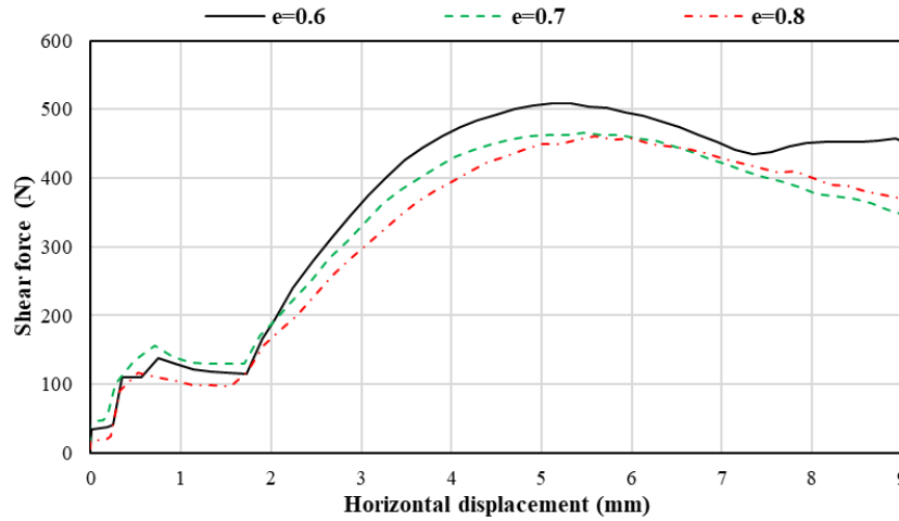
Figure 7. Relationship of shear force and horizontal displacement with different void ratio (dry sample, normal stress \sigma = 100 kPa, shearing rate 2.0 mm/min).
