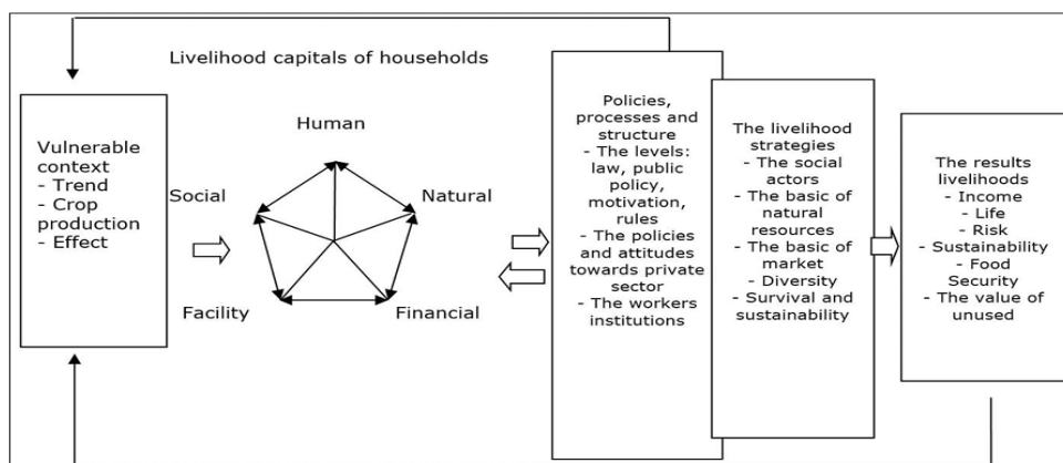
Figure 1. Sustainable livelihood framework (DFID 1999; Neefjes 2000)
