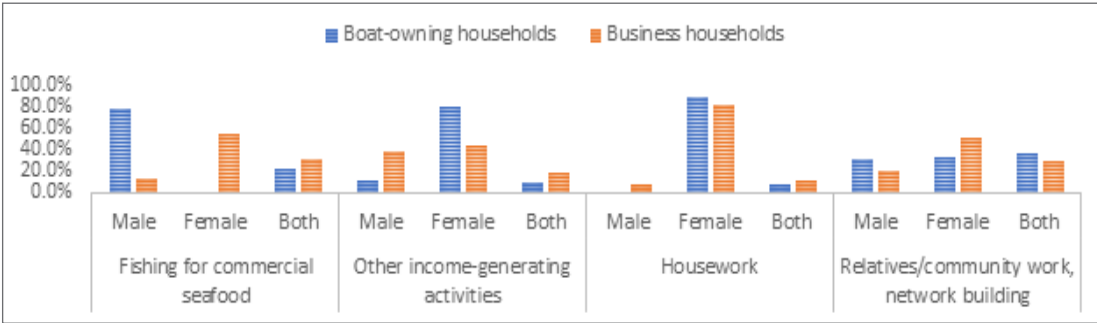
Figure 3. Decision-making power over key household activities (%) (N=157)
