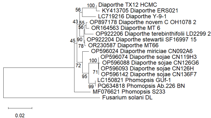
Figure 3. Phylogenetic relationships among the Diaporthe / Phomopsis strains. Numbers at the nodes are the bootstrapped values (in percent). The NCBI accession numbers are shown before the species names. F. solani DL sequence [25] was used as an outgroup.
