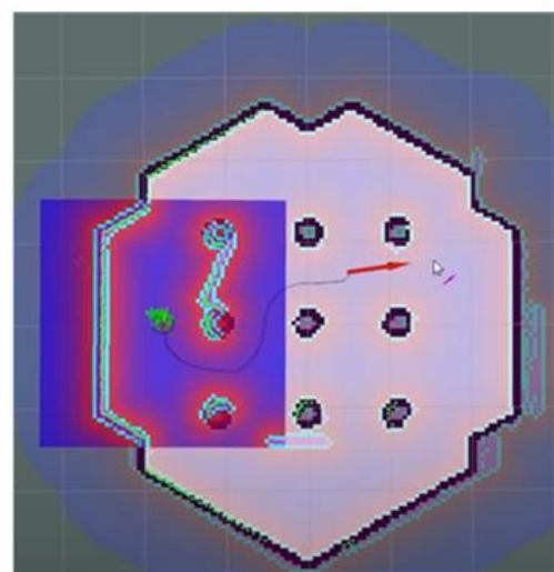
Figure 6. Robot is running to the goal with vertical obstacle
