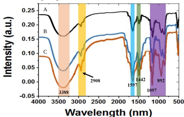
Figure 3. FTIR spectrum of magnetic biochar. (A) BCM-400; (B) BCM-500; (C) BCM-600.
