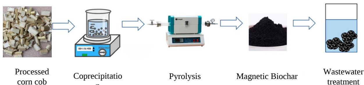
Figure 1. Process for synthesizing magnetic biochar
