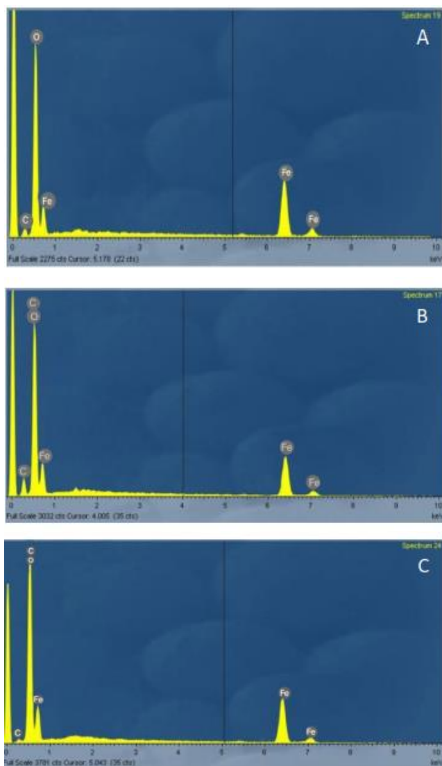
Figure 4. EDX results of biochar. (A) BCM-400; (B) BCM-500; (C) BCM-600.
