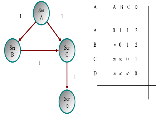
Fig. 2 Graph and distinct matrix
