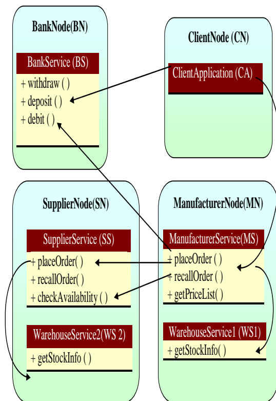
Fig. 5 Communication of Web-service when works with SOAP extension
