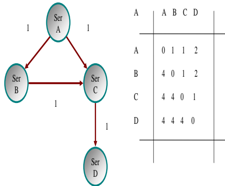
Fig. 3 Graph and distinct matrix with K=4
