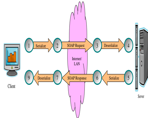
Fig. 5 Communication of Web-service when works with SOAP extension
