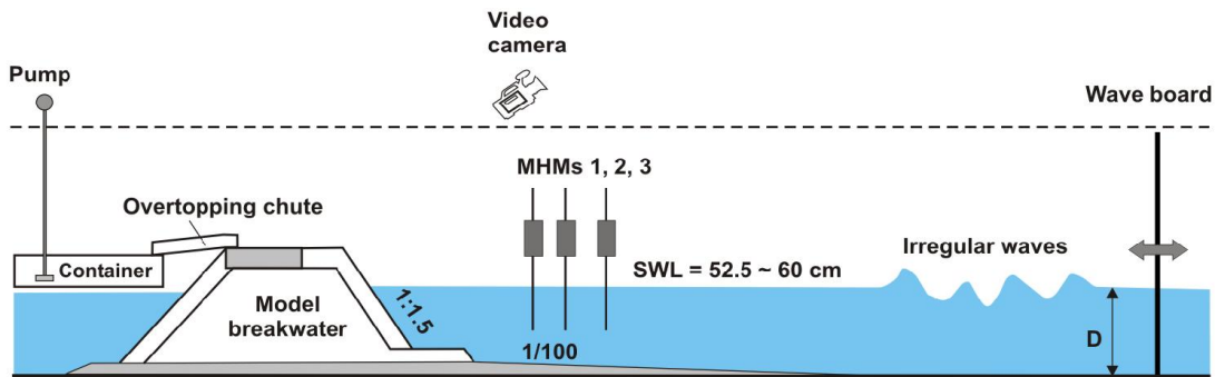
Fig 1. Experimental layout
