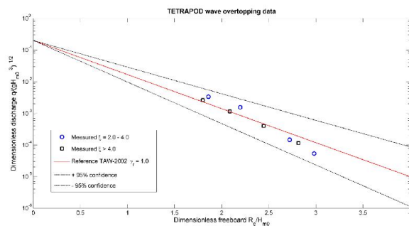
Fig 7. Wave overtopping data re-elaborated with roughness factors
