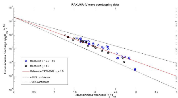
Fig 9. Wave overtopping data re-elaborated with roughness factors
