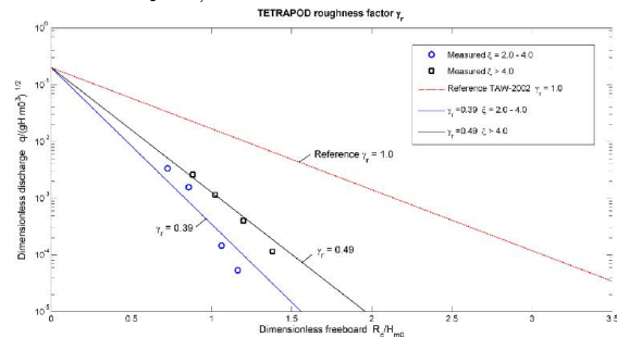
Fig 6. Roughness factor of Tetrapod
