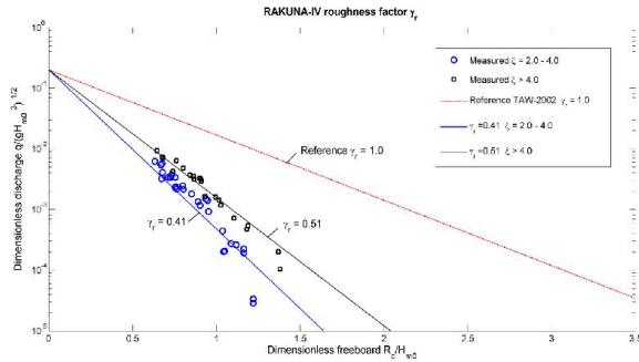
Fig 8. Roughness factor of Rakuna
