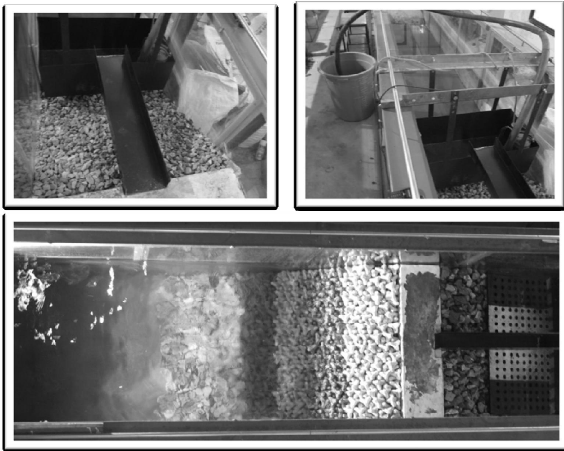
Fig 4. Overtopping chute and container
