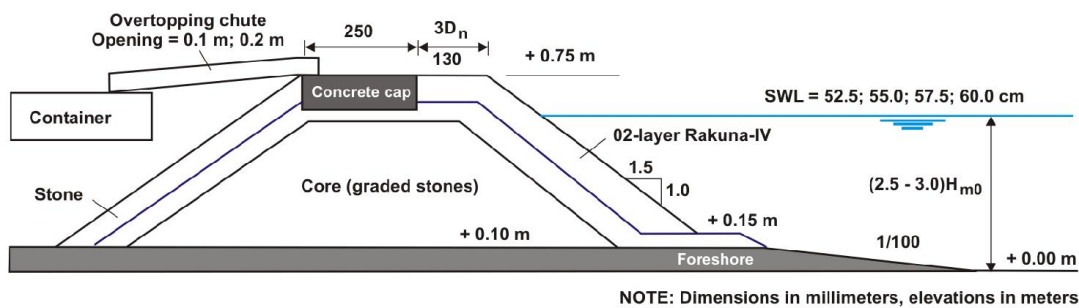
Fig 1. Experimental layout
