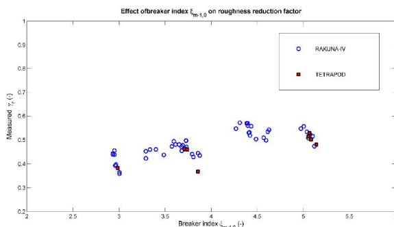
Fig 5. Variation of \gamma_r with \xi_{m-1,0}
