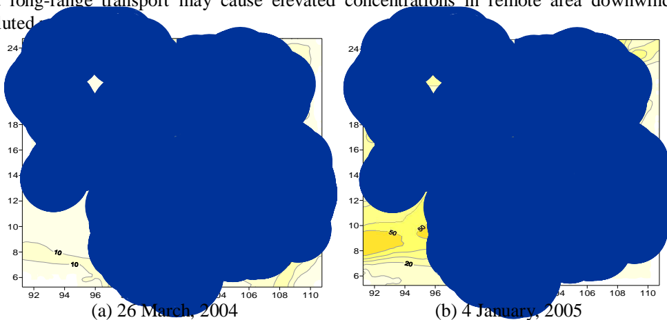
Figure 5. Modeled surface ozone distributions over CSEA domain at 7:00 UTC
