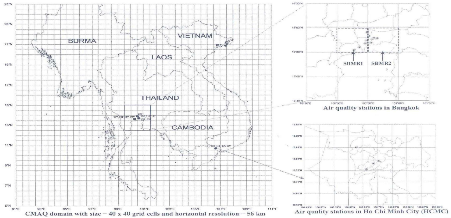
Figure 1. Model domain and location of air quality monitoring stations in CSEA domain (see also Table 1).
