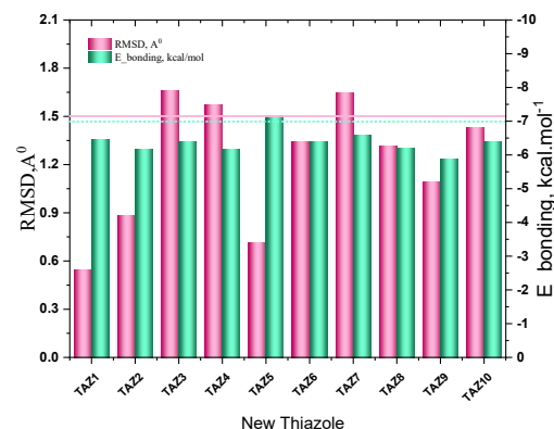
Figure 8. Docking results of 10 novel thiazole on PDB-3FC2
