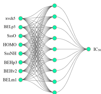
Figure 4. Architecture of neural network I(8)-HL(9)-O(1) model
