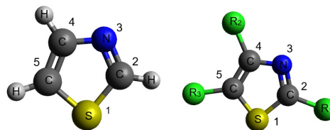
Figure 1. The Thiazole and its derivatives structure in the work
