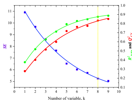
Figure 2. Change of values RMSE, R 2 train and Q 2 LOO according to k descriptors
