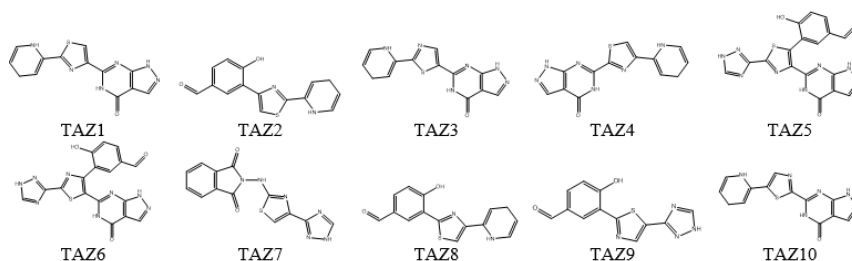
Figure 6. The structures of 10 novel thiazole derivatives
