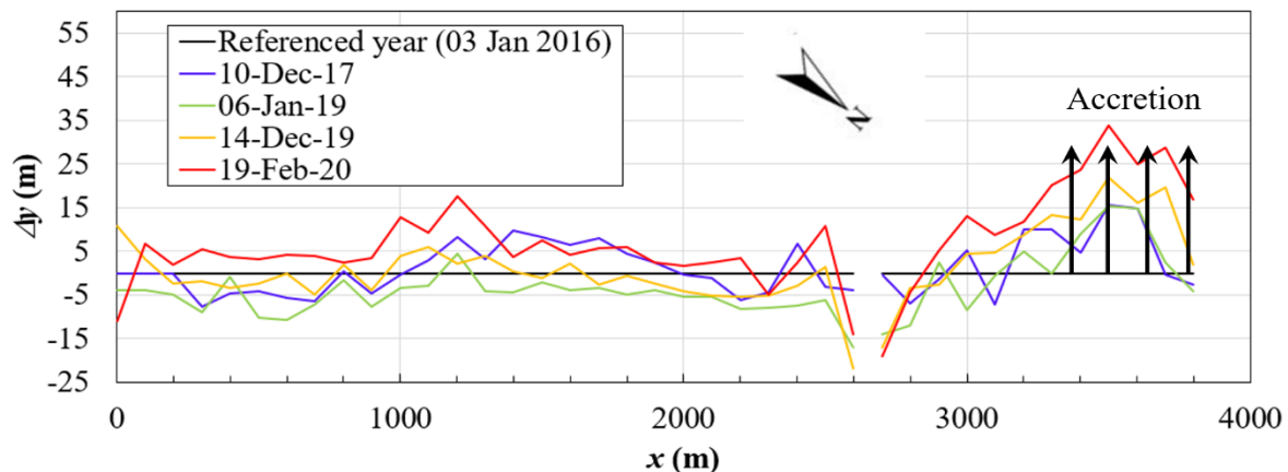
Figure 8. Shoreline changes.
