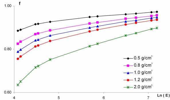
Fig. 6. The dependence of factor f on energy and density of soil matrix
