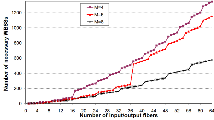
Figure 2. Number of required WBSSs
