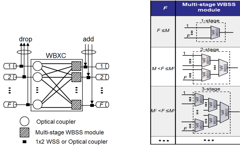
Figure 1. Proposed 1xM WBSS-based waveband cross-connect architecture
