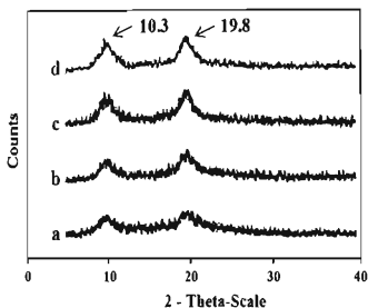
Figure 3. XRD patterns of the initial (a) and degraded chitosan in swollen state with 1 % (b), 3 % (c) and 5 % (d) concentration of H_2O_2 irradiated at 10 kGy.
