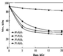
Figure 1. The molecular weight of chitosan versus treatment dose (the dose rate 3.6 \text{ kGy/h} )
