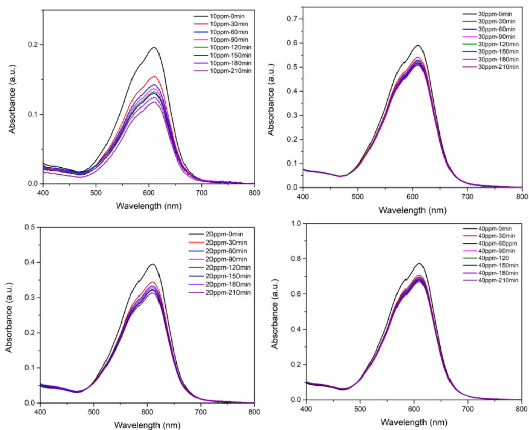
Figure 11. Absorbance with modified coal NaOH 1.5 M
