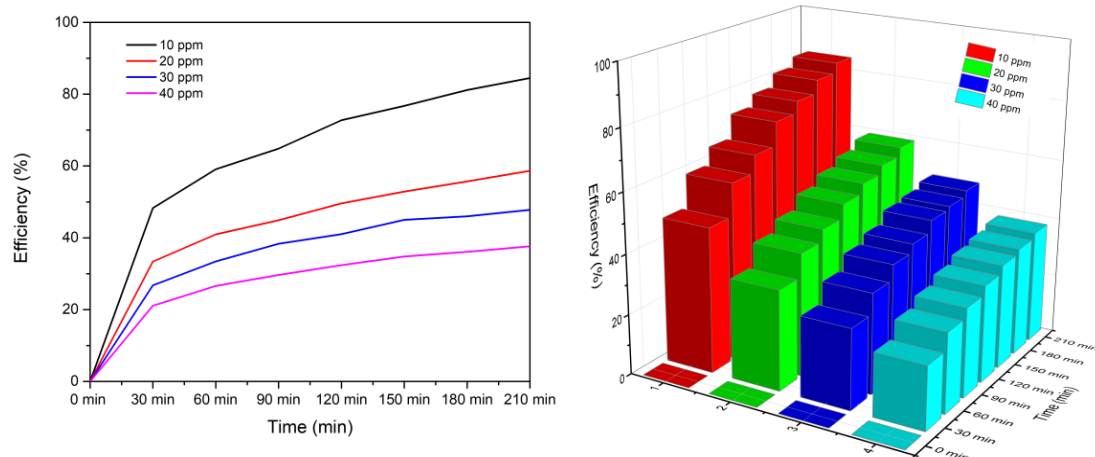
Figure 10. Efficiency with modified coal NaOH 1M
