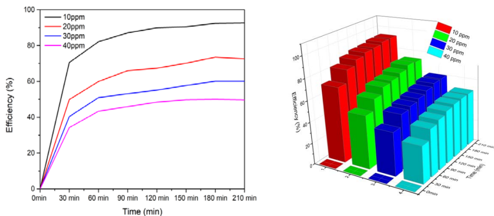
Figure 14. Efficiency with modified coal NaOH 2M
