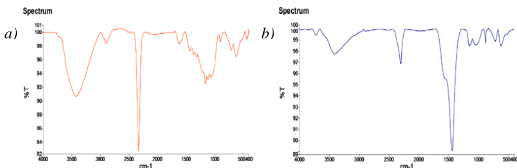
Figure 2. a) FT-IR of AC before processing . b) FT-IR of AC after processing
