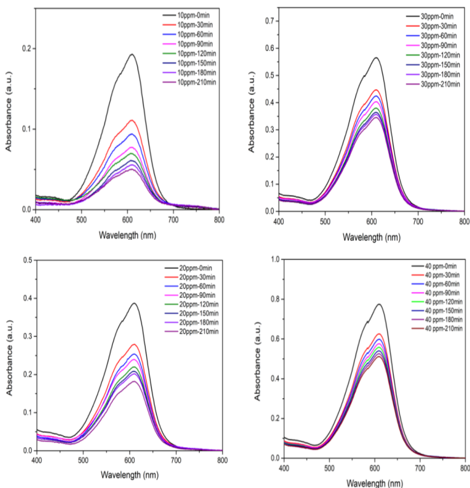
Figure 16. Absorbance with one-time regenerated activated carbon
