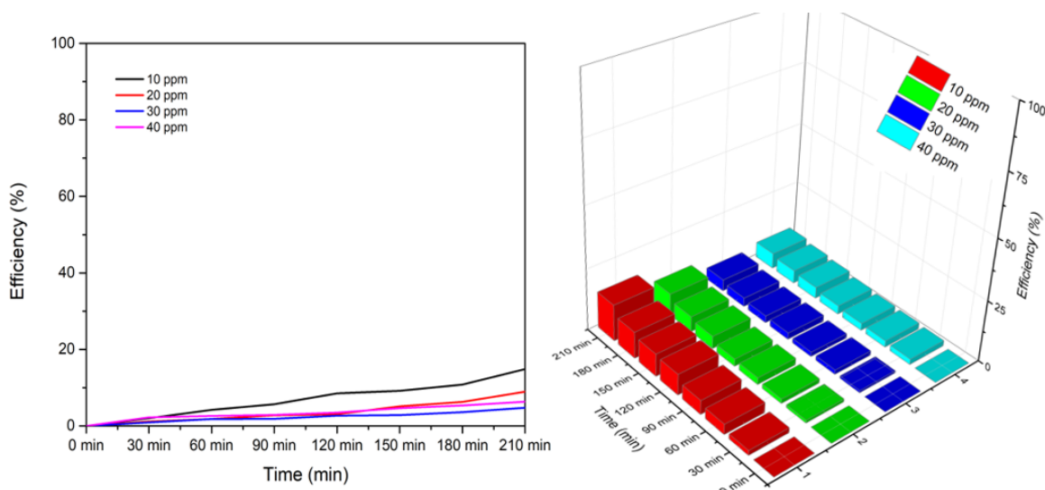
Figure 8. Efficiency with unmodified charcoal
