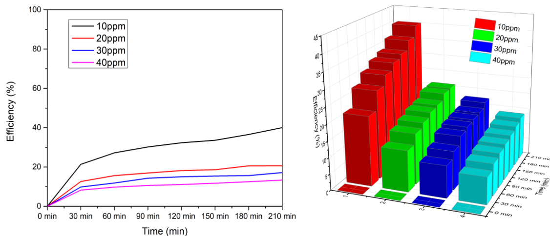
Figure 12. Efficiency with modified coal NaOH 1.5M
