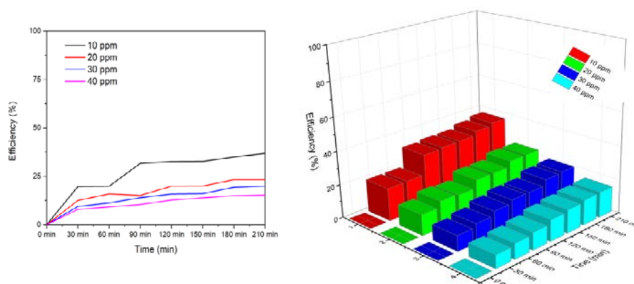
Figure 17. Efficiency with one-time regenerated activated carbon
