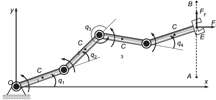
Fig. 1. A redundant four-link planar manipulator
