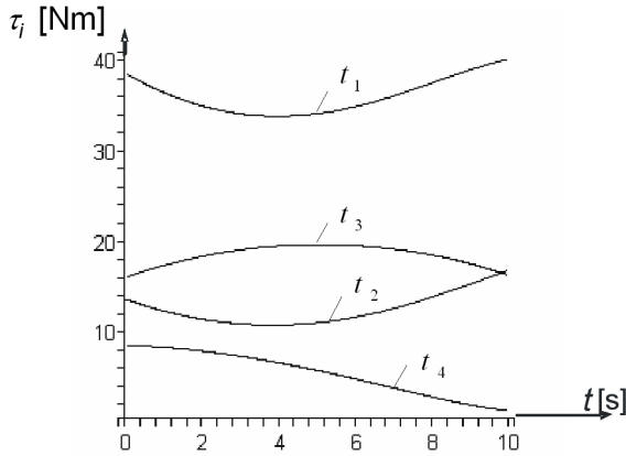
Fig. 2. Joint torques versus time for the first case
