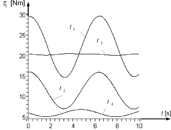
Fig. 4. Joint torques versus time for the second case
