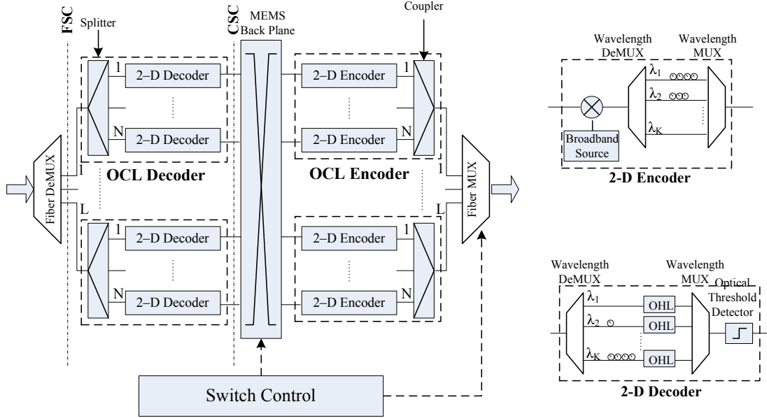
Figure 2. Architecture of core GMPLS switch using 2-D code label
