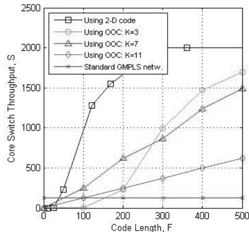
Figure 4. Core switch throughput (S) versus code length (F) when the number of input flows ( N_f ) is 2000 and the packet length (X) is 1024
