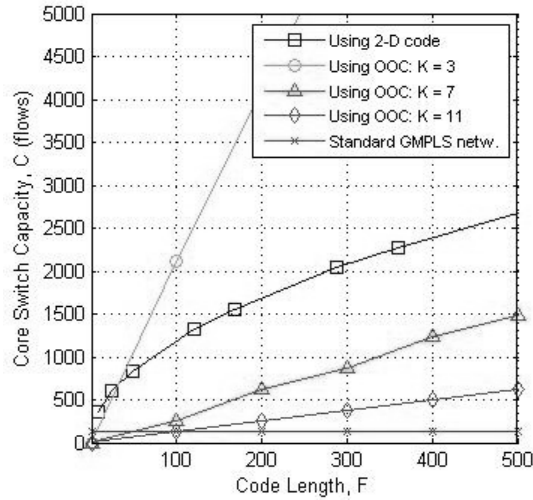
Figure 3. Core switch capacity ( C ) versus the code length ( F ) when the number of fibers L is 4 and the number of wavelengths M is 31
