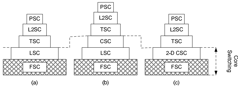
Figure 1. Label mapping layers in GMPLS networks
