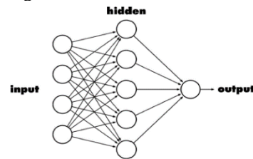
Figure 1: ANN structure
