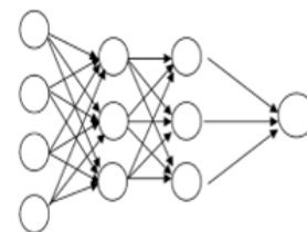
Figure 2: Feed-forward ANN
