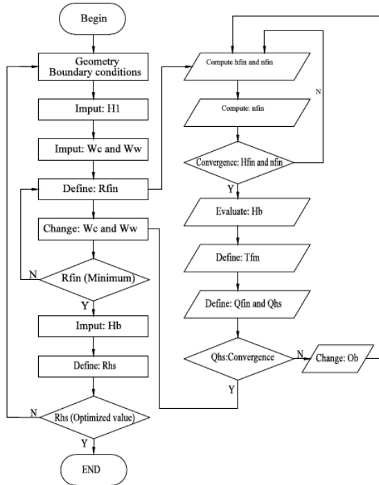
Figure 4: Optimal heatsink fins calculation.
