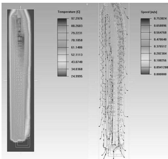
Figure 10: Thermal simulation results.
