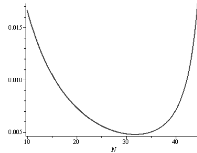
Figure 7: Optimal number of fins [2].
