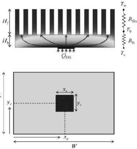
Figure 3: The heat sinks with heat source.
