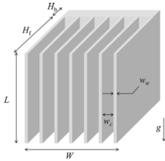
Figure 2: Input parameters of heatsink [2].
