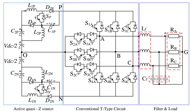
Figure 2: The topology of 3L-AqZS-T 2 I.
