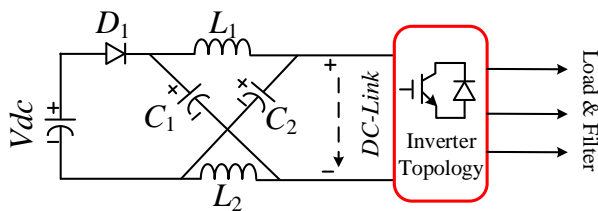
Figure 1: The Z-Source impedance network topology.
