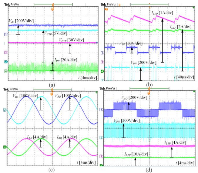
Figure 11: Experimental results for 200V input voltage.
