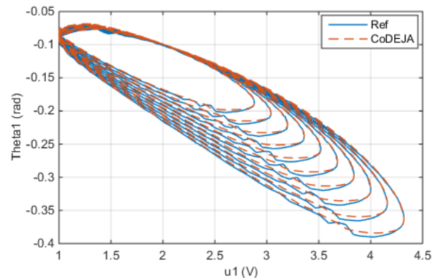
Figure 13: The performance identification curve of PMA system
