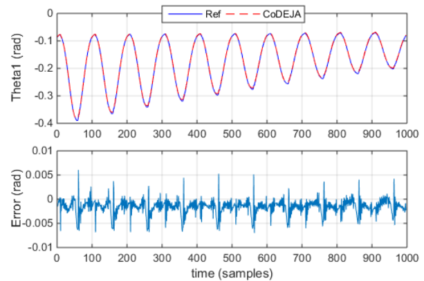
Figure 11: Performance identification of PMA system
