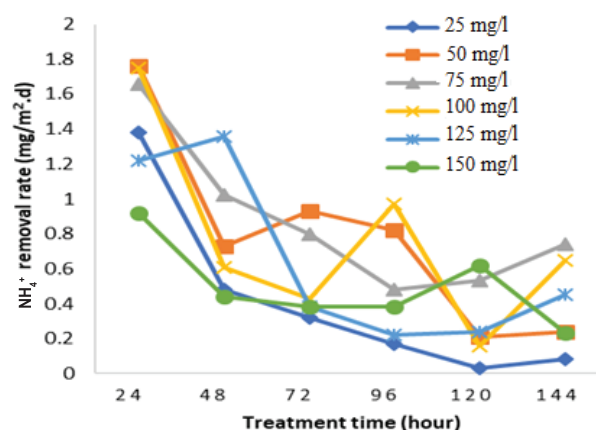
Fig. 9. The \text{NH}_4^+ removal rate by HSF CWs planted with Cyperus alternifolius during the experiment.
