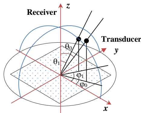
Figure 1. The configuration for ultrasonic computer tomography.
