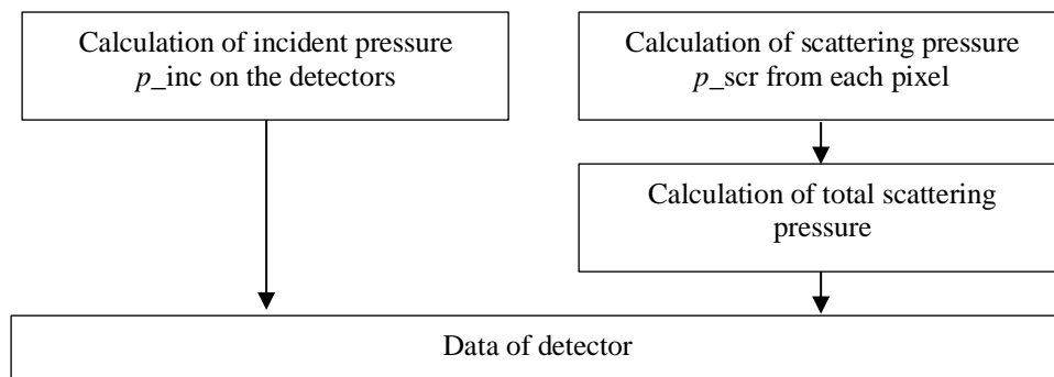
Figure 2. The follow chart of computation.
