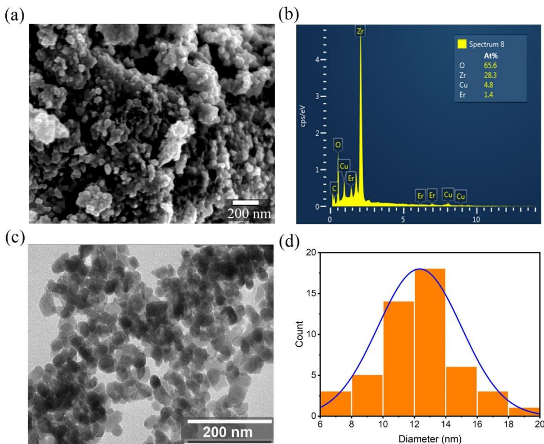
Figure 3. (a) SEM image, (b) EDS spectrum, (c) TEM image and (d) particle size distribution of ZrO 2 /CuO doped with 5 mol% Er 3+
