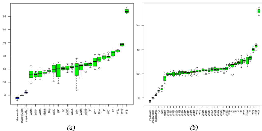
Figure 6. Boruta plot of the wind speed: (a) Basel and (b) Osaka Table 3. Summary the rank of features in two cities
