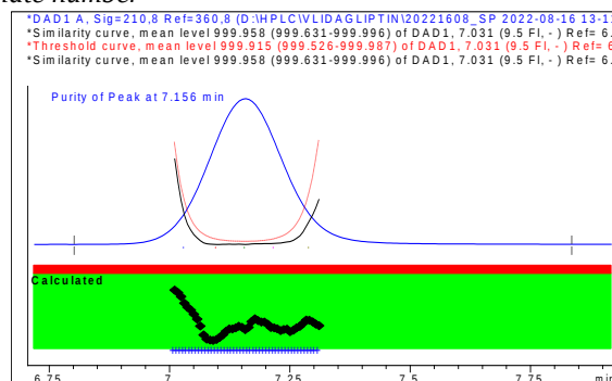
Figure 5. Purity of the vildagliptin peak in the specificity test
