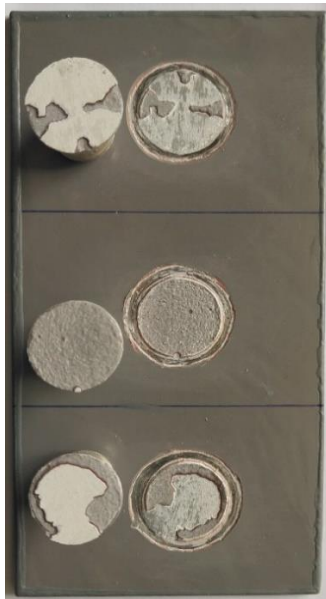
Figure 5a. Image of destruction on first coating (sample TMP2)
