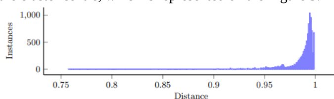
Figure 3. The histogram chart illustrates the number of images based on the distances between images and their neighbours after removing duplicate images.
