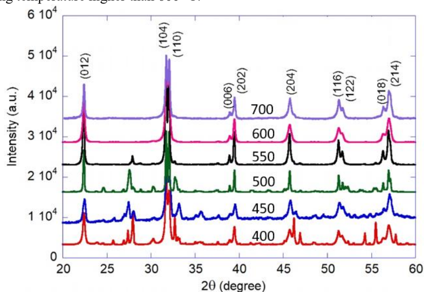
Figure 1. XRD profiles of BFO synthesized at different annealing temperatures
