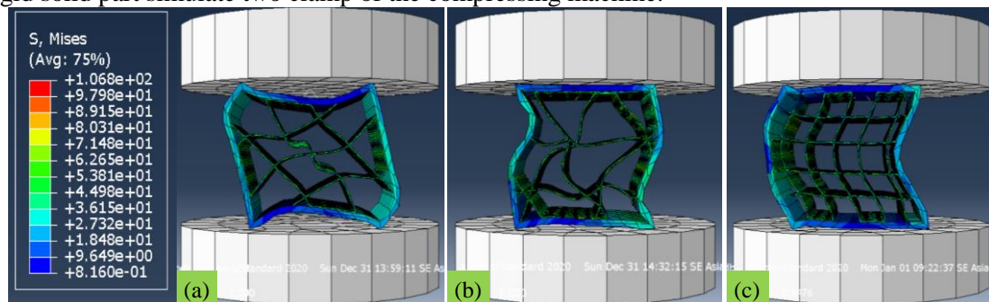
Figure 4. Von Mises stress and deformed shapes of: (a) Grid 45 CCF model; (b) Triangle CCF model; (c) Grid 90 CCF model
