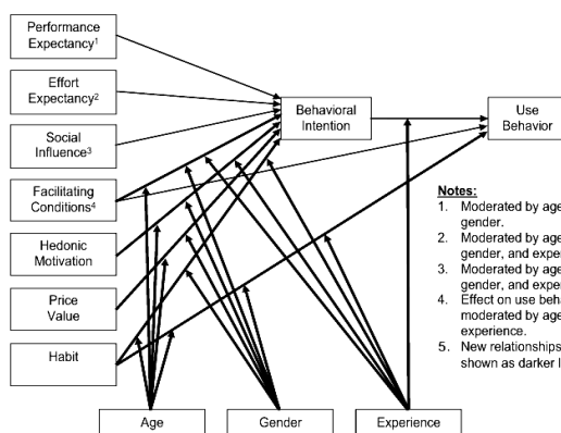
Figure 1. UTAUT2
