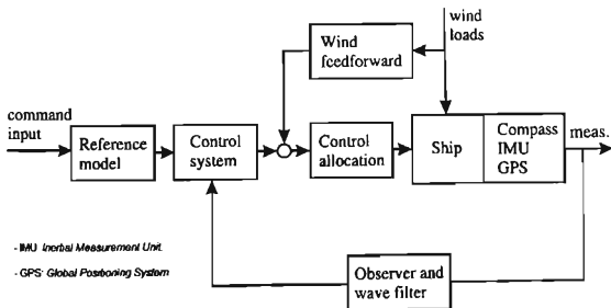
Fig. 1. Typical control structure of ships
